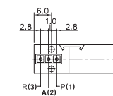
YSV11-DP-L-*** Normally Open Type
